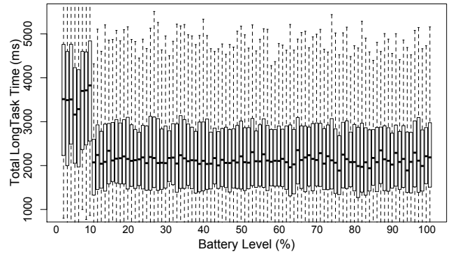
Figure 7: LongTask time distributions across different device battery charge levels, as measured for a page loaded on P8 Lite (2015) smartphone.
