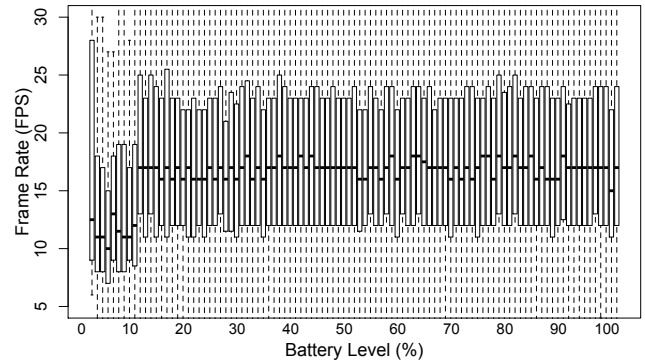
Figure 9: FPS distributions across different device battery charge levels, as measured for a page loaded on P8 Lite (2015) smartphone.
